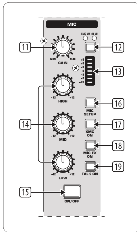
Fig. 8: Microphone channel
